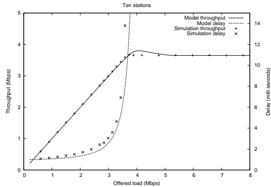
Fig. 2. Symmetric network throughput and delay. Model predictions and NS simulations.
