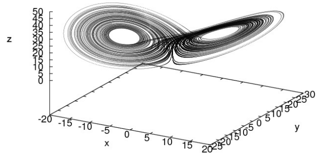
Figure 1: The Lorenz attractor
