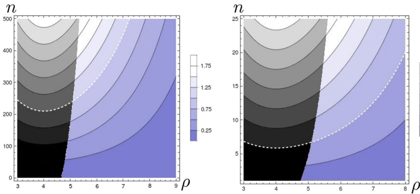
Fig. 4 Many obstacles: Taking the Sinai-like domain in Fig. 1 with side L = 100 and containing n circular obstacles of small radii r = 1 (left-hand phase diagram) and large radii r = 6 (right-hand phase diagram), we plot the ratio of the first term in Eq. 5.2 with the sum of the components in Eq. 5.1, whose magnitude is indicated by the color gradient on the respective legend. The obstacle effects dominate when this exceeds unity, highlighted by the dotted line on each graph. Also, the regions where P_{fc} is (predicted by our formulas to be) below 4/5 are faded to gray tones, indicating regions where our approximations to the connection probability begin to lose their accuracy. \beta = 1 throughout
