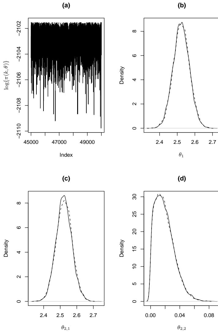
Figure 1: MCMC output for example problem: (a) Trace of log posterior for last 5 000 sweeps of sampler; (b) density estimate for \theta_1 when k = 1 ; (c) density estimate for \theta_{2,1} when k = 2 ; and (d) density estimate for \theta_{2,2} when k = 2 . Solid lines are problem specific sampler of section 3.1, dashed lines are AutoMix sampler of section 5.
