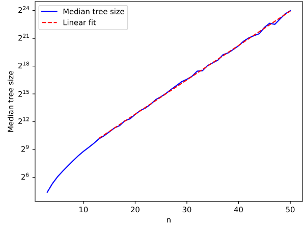
Figure 4. Median tree size explored by classical branch-and-bound algorithm with depth-first strategy. 99 random instances generated for each n . Fit is line y = 2^{0.371n+5.380} .
