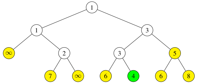
FIG. 1. An example tree corresponding to a branch-and-bound algorithm. Nodes are labelled with their cost bounds, which are non-decreasing on any path from the root to a leaf. The green node is the optimal solution; yellow nodes are removed if the tree is truncated at the optimal cost.
