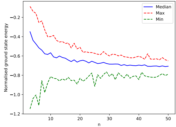
Figure 5. Normalised ground state energy E_{\min} n^{-3/2} of instances of the S-K model. 99 random instances generated for each n .
