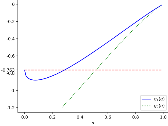
Figure 2. The functions g_1(\alpha), g_2(\alpha) defined in (C5), (C8). g_1(\alpha) \geq -0.763 for all \alpha \geq 0.4 , while g_2(\alpha) \geq -0.763 for all \alpha \geq 0.9 .
