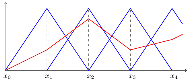
FIG. 1. A basis set of “tent” functions (blue), for piecewise linear functions defined on the line (an example of which is in red). Any piecewise linear function can be uniquely specified as a sum of scaled tents.
