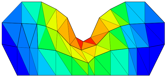
FIG. 2. An example of a “mesh” – a discretisation of the domain over which the PDE is defined. Each polygon is a “finite element”, with basis functions defined upon them. The colour scheme here represents the amplitude associated with the function supported on each finite element. As a physical example, the diagram could represent the material stress on a plate, induced by a deformation by a rod.
