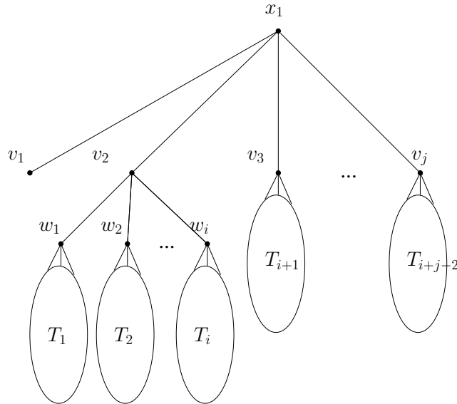
Figure 3: The second type of tree in Case 3.
