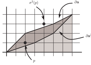
FIGURE 3. A point p and its shift p^{(2)} .
