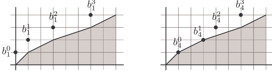
FIGURE 5. Construction of B_1 = \{b_1^j\} and B_4 = \{b_4^j\} relative to \mathbf{a} = (1, 2, 3, 2) .
