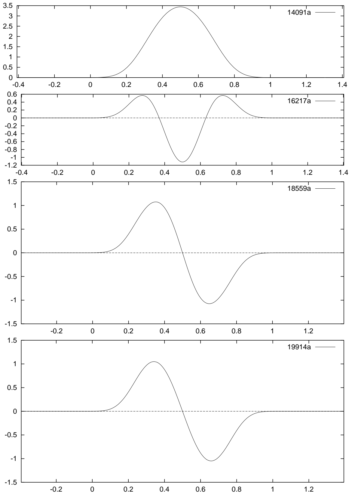
Figure A.2: S^*(N^\sigma) for genus 2 curves over \mathbb{Q} (cont.)
