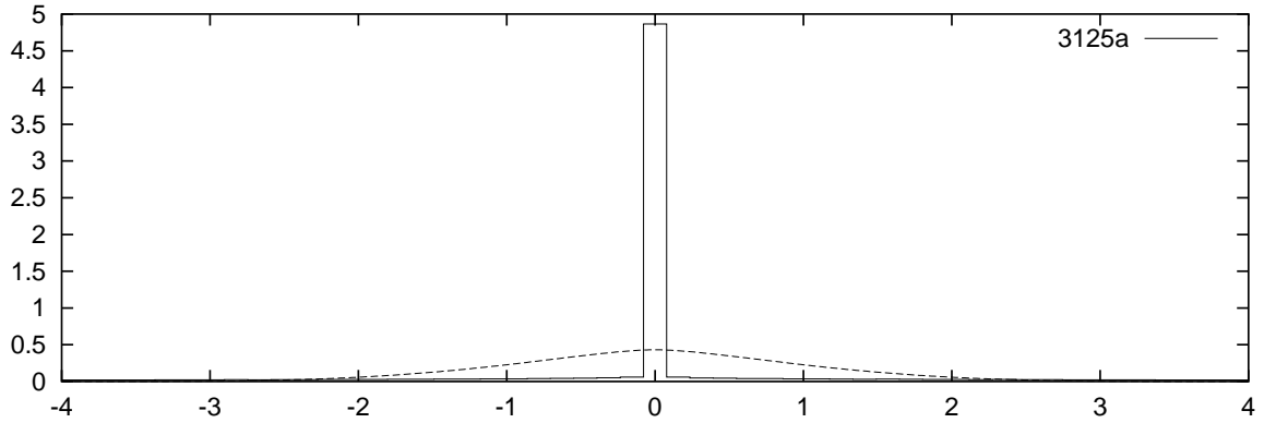
Figure 2.2: Distribution of Fourier coefficients for genus 2 curve 3125a
