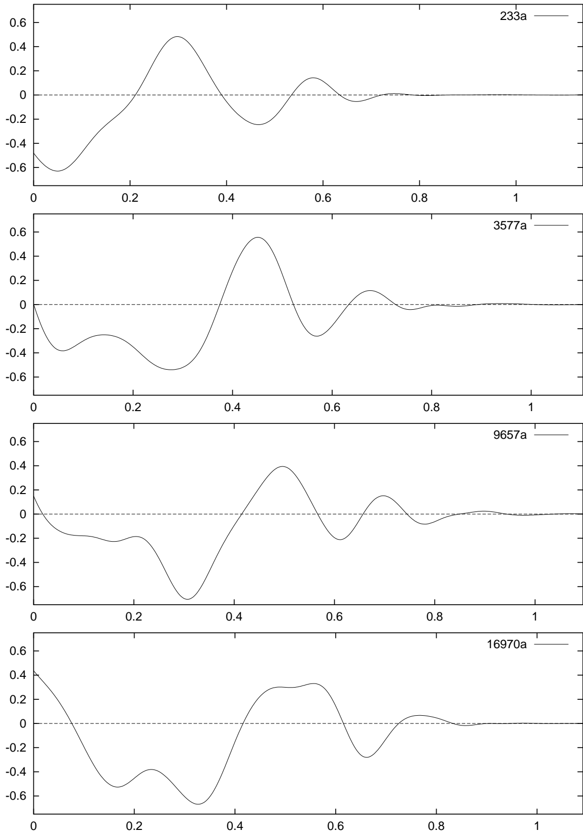
Figure 3.2: S(D^\sigma) for elliptic curves over \mathbb{Q}(\sqrt{-1})
