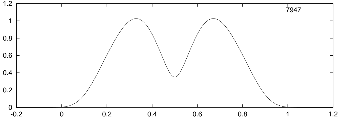
Figure 7.1: |S^*(N^\sigma)| for the Galois representation \rho of conductor N = 7947
