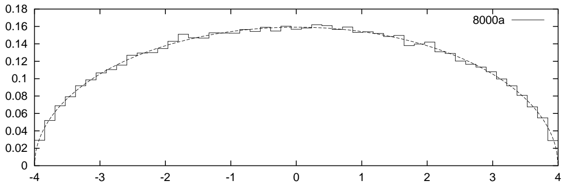
Figure 2.3: Distribution of Fourier coefficients for elliptic curve 8000a, compared with a stretched Sato-Tate measure
