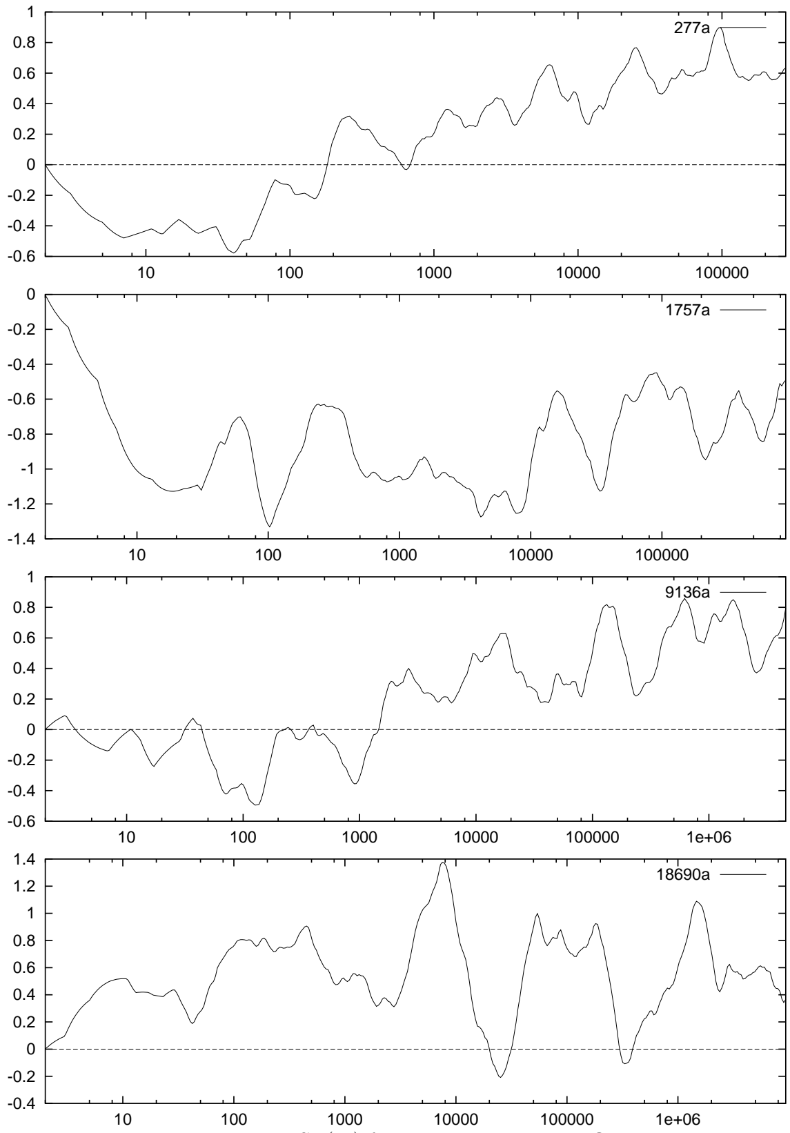
Figure 3.3: S^{\text{pr}}(X) for genus 2 curves over \mathbb{Q}
