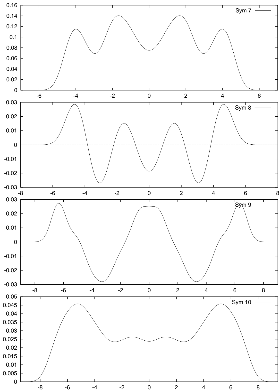
Figure 7.3: S^*(e^\sigma) for \text{Sym}^n \Delta
