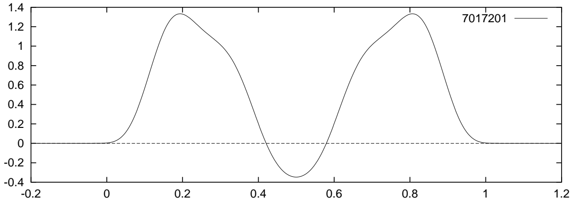
Figure 7.2: S^*(N^\sigma) for the self-dual twist \tilde{\rho} of conductor N = 7017201
