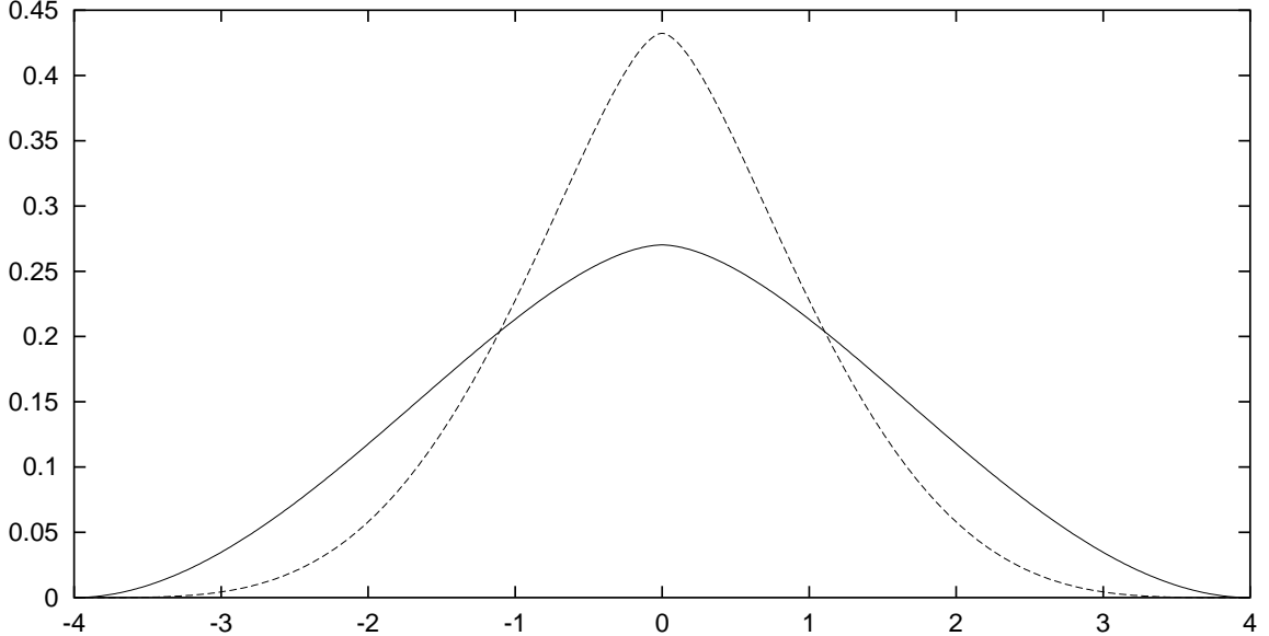
Figure 2.1: Expected distributions of Fourier coefficients \lambda_E(p) for p \equiv 1 \pmod{4} (solid line), and \lambda_C(p) for all primes (dashed line)
