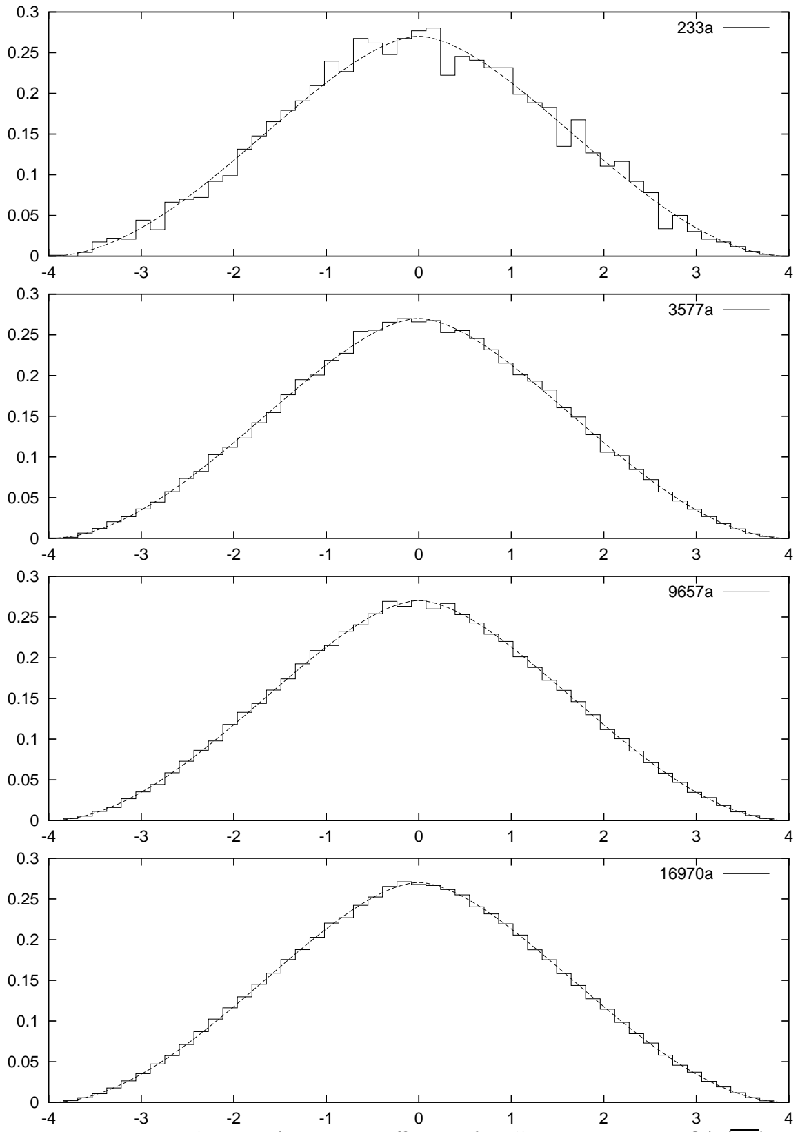
Figure 2.5: Distribution of Fourier coefficients for elliptic curves over \mathbb{Q}(\sqrt{-1})
