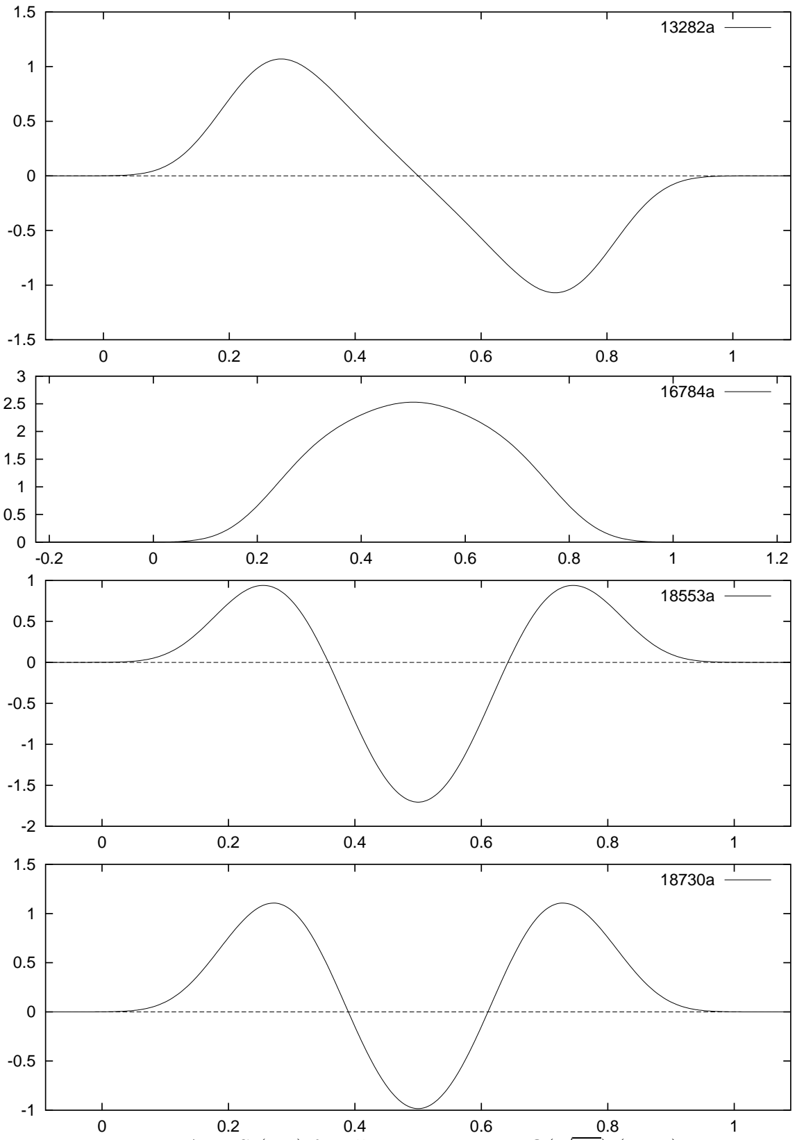
Figure A.4: S^*(N^\sigma) for elliptic curves over \mathbb{Q}(\sqrt{-1}) (cont.)
