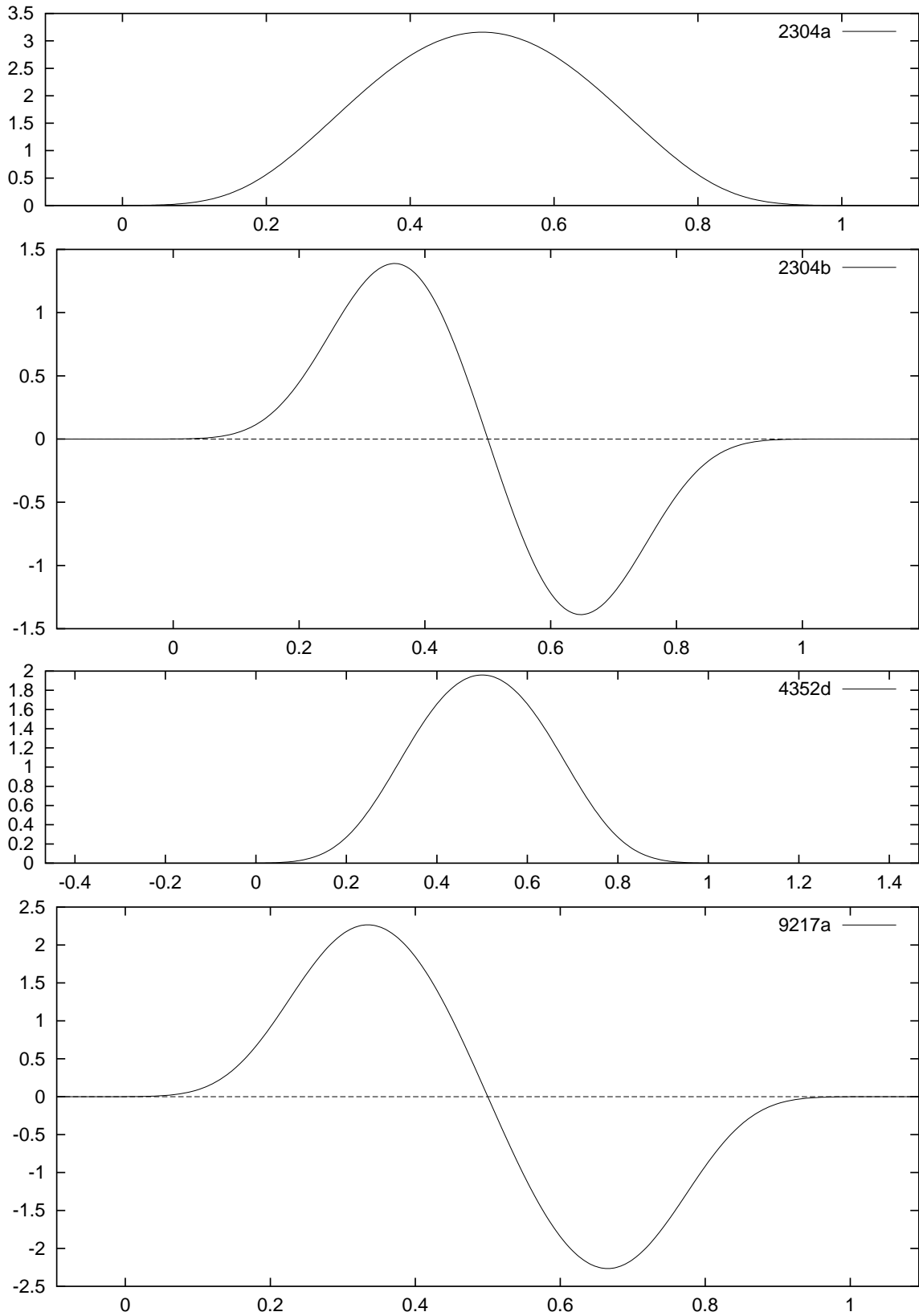
Figure A.3: S^*(N^\sigma) for elliptic curves over \mathbb{Q}(\sqrt{-1})
