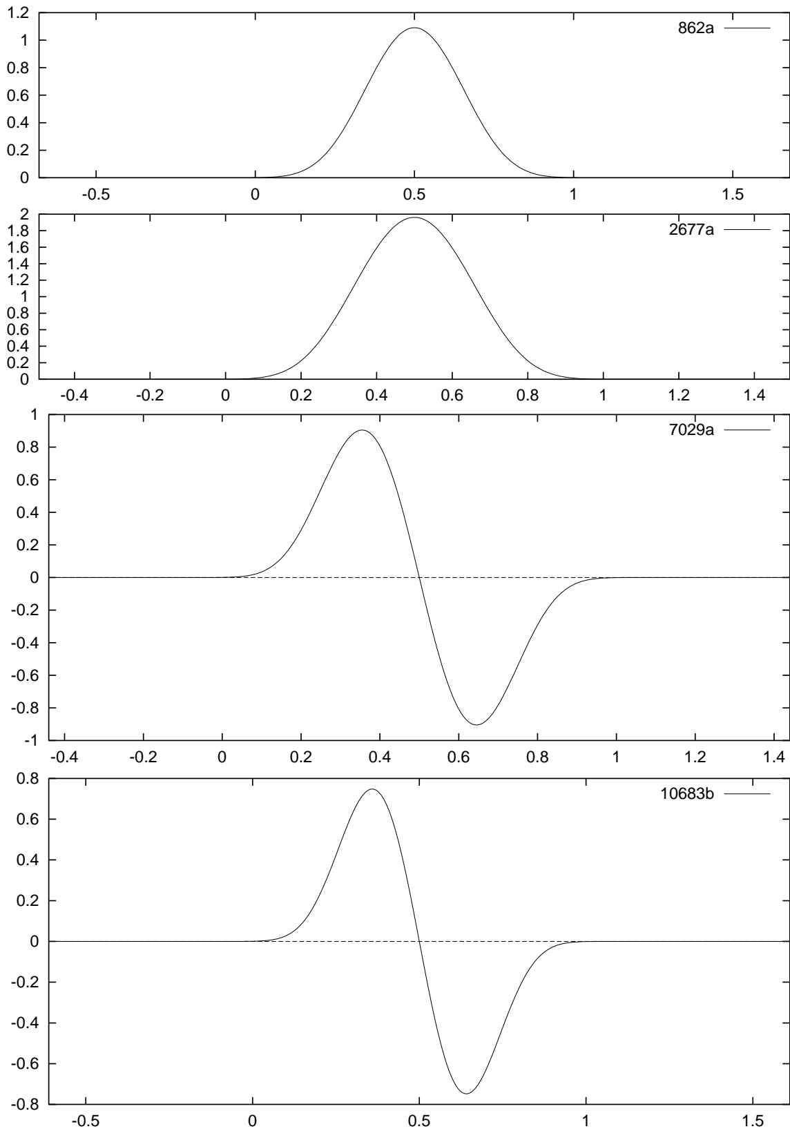
Figure A.1: S^*(N^\sigma) for genus 2 curves over \mathbb{Q}
