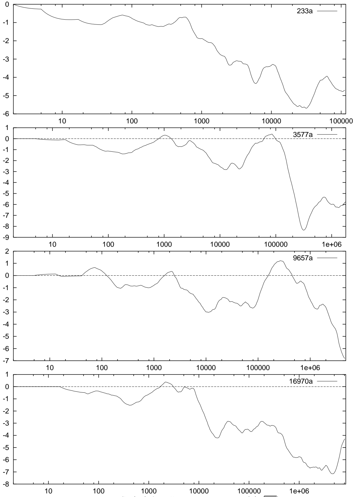
Figure 3.4: S^{\text{pr}}(X) for elliptic curves over \mathbb{Q}(\sqrt{-1})
