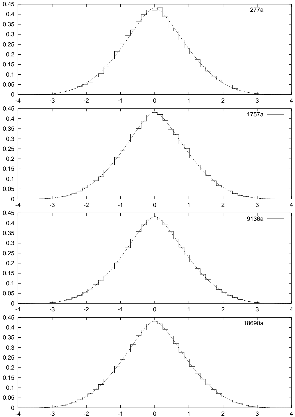
Figure 2.4: Distribution of Fourier coefficients for genus 2 curves over \mathbb{Q}
