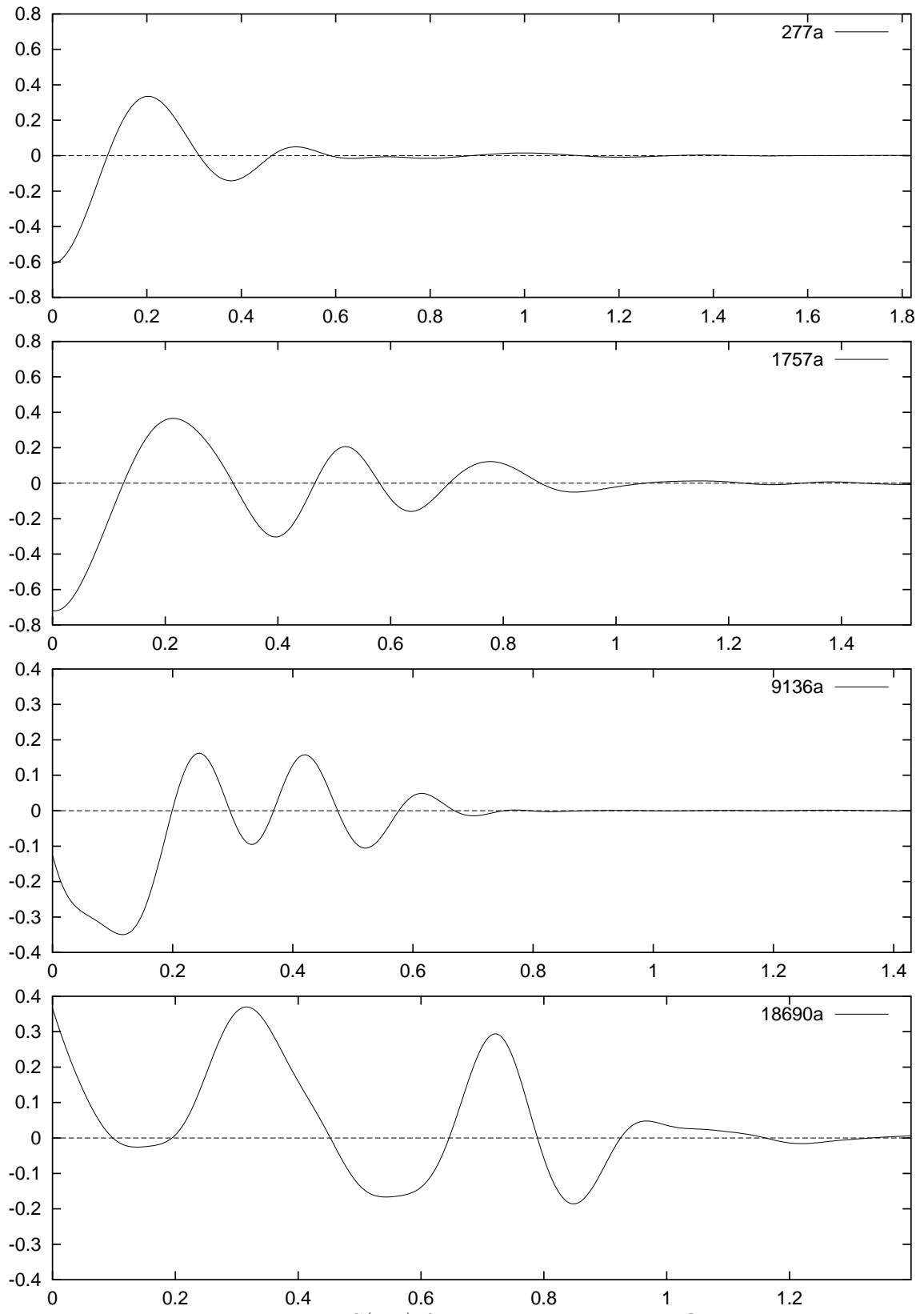
Figure 3.1: S(D^\sigma) for genus 2 curves over \mathbb{Q}
