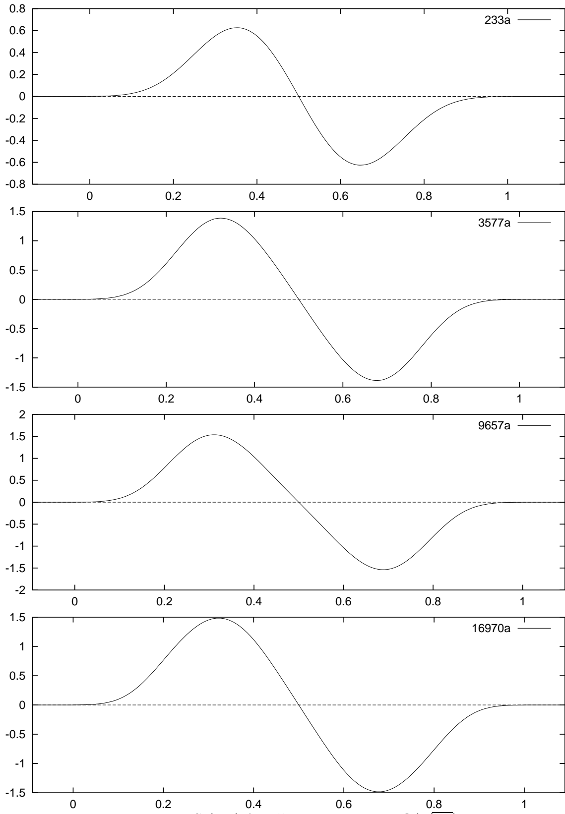
Figure 5.2: S^*(N^\sigma) for elliptic curves over \mathbb{Q}(\sqrt{-1})
