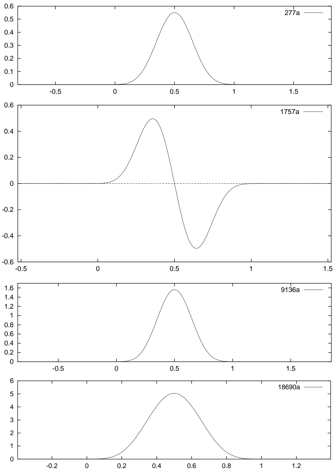
Figure 5.1: S^*(N^\sigma) for curves of genus 2 over \mathbb{Q}
