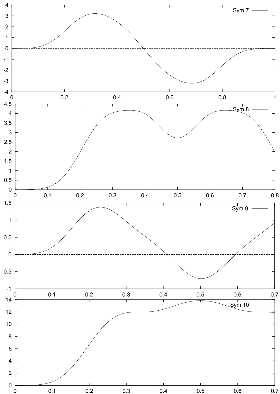
Figure 7.4: S^*(N^\sigma) for \text{Sym}^n f of conductor N = 11^n
